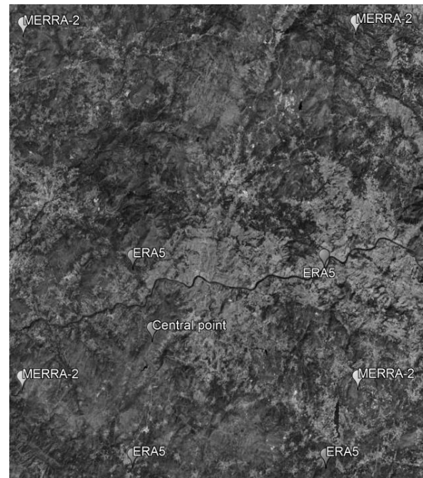
Fig. 2. Representation of the central point of a certain wind farm and the respective extracted reanalysis points.
