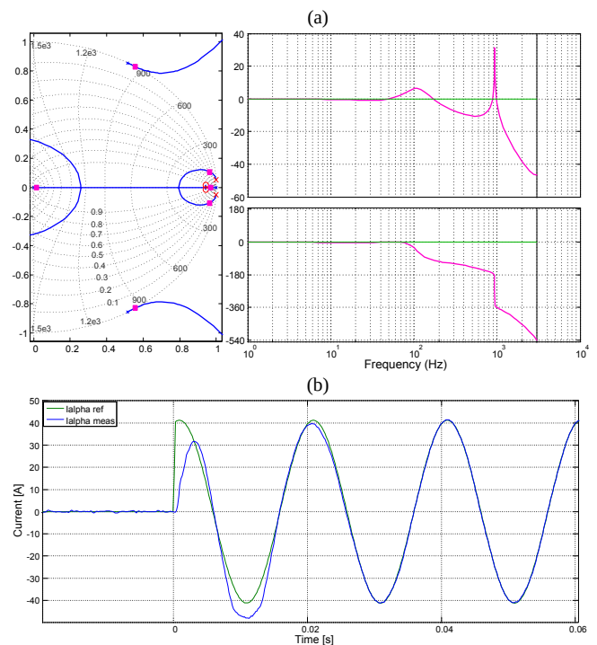
Fig. 5. (a) Root-locus and closed loop pole response for 50Hz current control design parameters. (b) Current alpha reference and measured obtained in the experimental results
