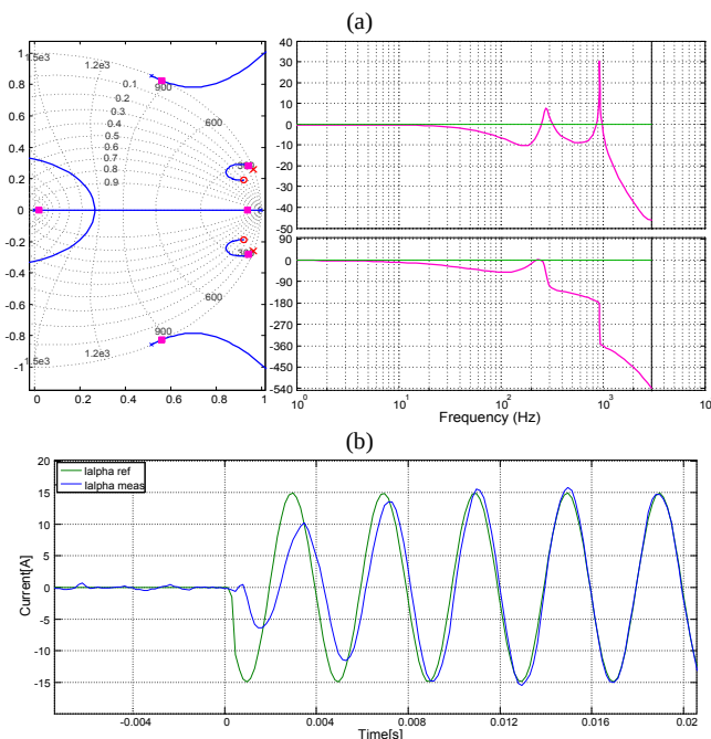
Fig. 6(a) Root-locus and closed loop pole response for 250Hz current control design parameters. (b) Current alpha reference and measured obtained in the experimental results
