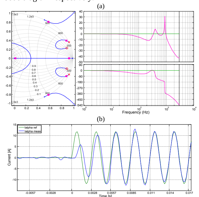
Fig. 7(a) Root-locus and closed loop pole response for 350Hz current control design parameters. (b) Current alpha reference and measured obtained in the experimental results
