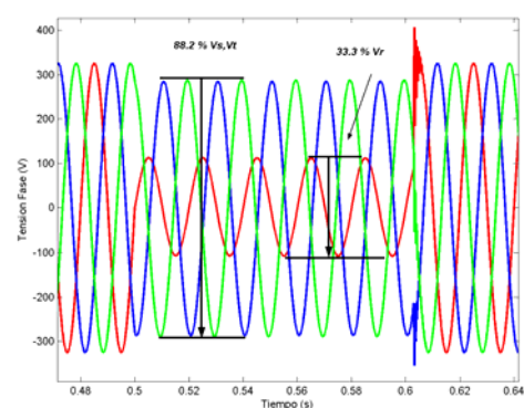
Fig. 2. Voltage waveform.
