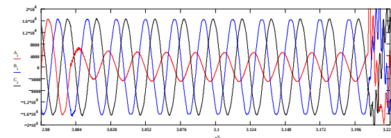
Fig.15.Phase voltages during a type D_R sag at the 22 kV bus
