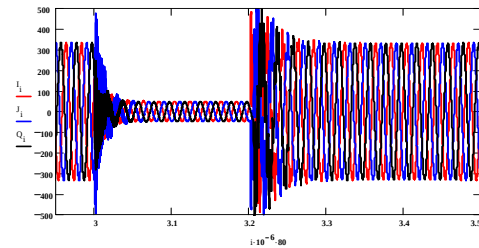
Fig.11.Phase voltages at the 400 V bus. Sag A propagated down from 22 kV bus is an A sag at 400 V
