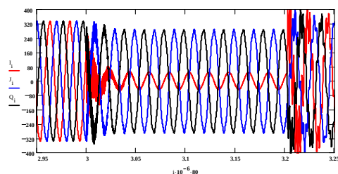
Fig.13.Phase voltages at the 400 V bus.
