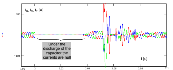
Fig 21. Line currents during the sag event
