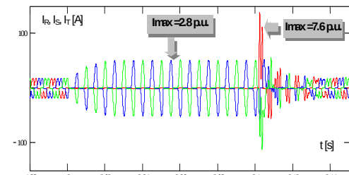
Fig 24. Line currents during the sag event
