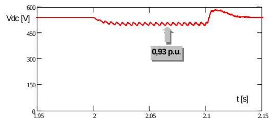
Fig 25. Decrease of the DC bus voltage under sag
