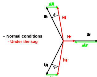
Fig 5. Three-phase phasor diagram during and before the sag
