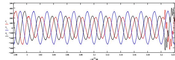
Fig. 16.Phase voltages at the 400 V bus. Sag D_R propagated down from 22 kV bus is a C_S sag at 400 V
