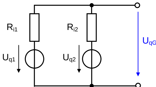
Fig. 13. Parallel connection of TEG modules with different temperature differences.
