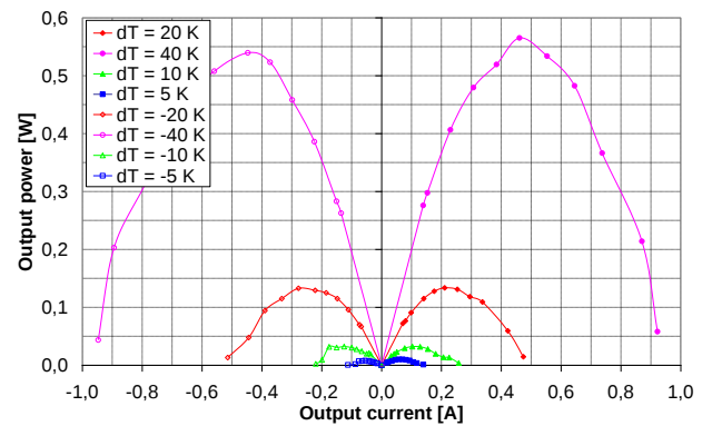
Fig. 5. Output power and current of GM250-127-14-16 for several temperature differences between cold side and hot side.
