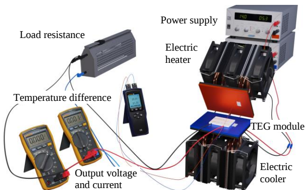
Fig. 3. Experimental setup.
