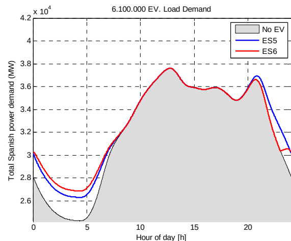
Fig.12. Total load demand NoEV-ES5-ES6 (2019)
