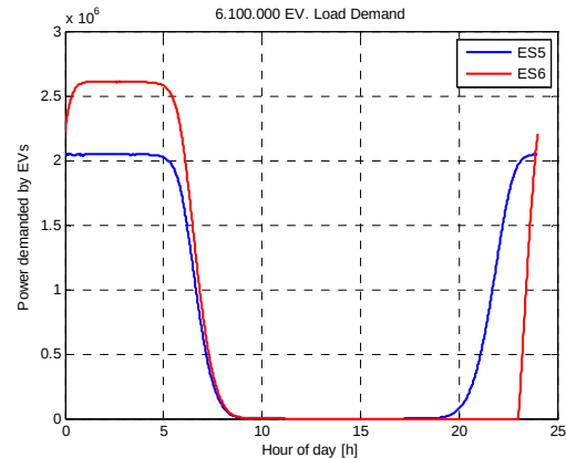
Fig.11. Power demanded by electric vehicles (ES5-ES6)
