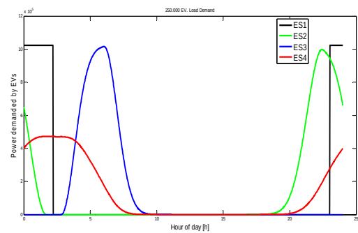
Fig.6. Power demanded by electric vehicles (ES1-ES4)
