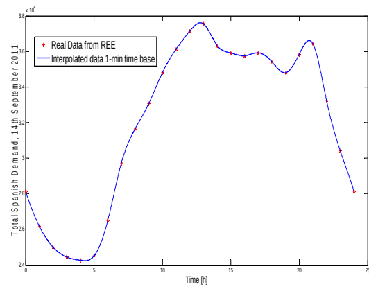
Fig. 1. Summer load profile for the mainland Spanish system
