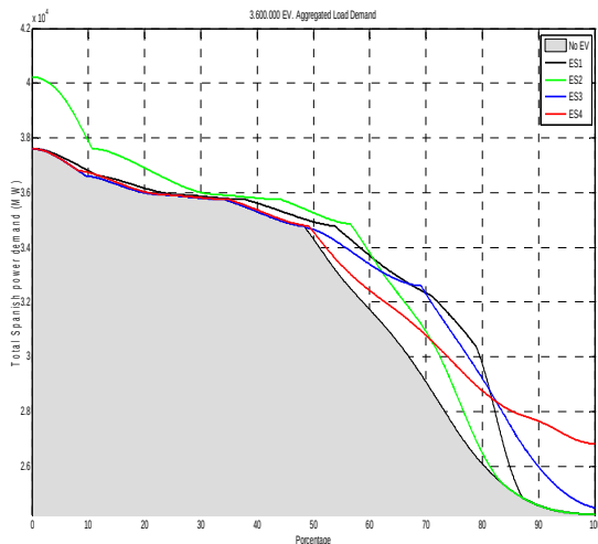
Fig.10. Aggregated Load demand NoEV-ES1-ES2-ES3-ES4 (2017)
