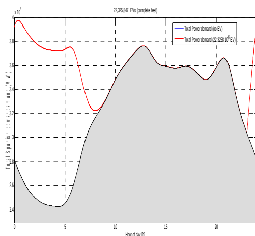
Fig.13. Total load demand NoEV- ES6 MAX
