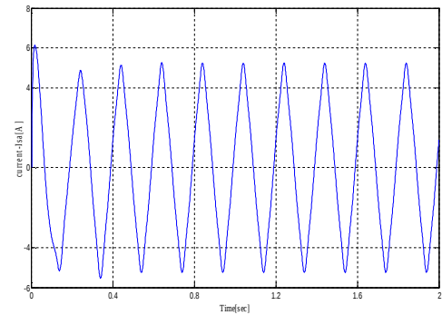
Fig.5 Phase stator current without HF signal injection
