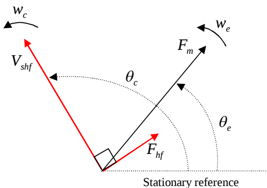
Fig.2 Low and high frequency fields' relation
