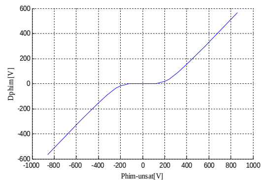
Fig.1 Curve \Delta\bar{\Psi}_m = f(\bar{\Psi}_{m,unsat})
