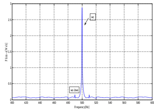
Fig.11 Spectrum of Magnetizing flux \lambda_{m-a} with HF signal injection
