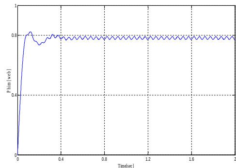
Fig.7 Magnetizing flux without HF signal injection
