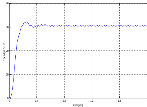
Fig.3 Speed response without HF signal injection
