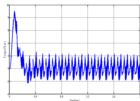
Fig.15 Electromagnetic Torque response with HF signal injection
