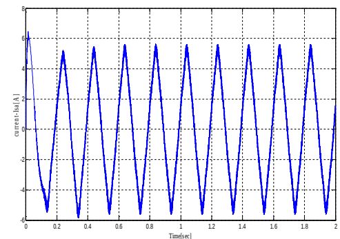
Fig.13 Phase stator current with HF signal injection
