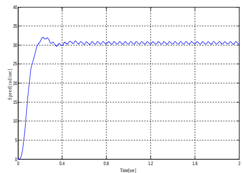
Fig.12 Speed response with HF signal injection
