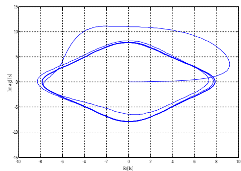
Fig.6 Phase stator current trajectory
