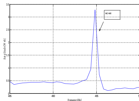
Fig.10 Spectrum of Magnetizing flux with HF signal injection
