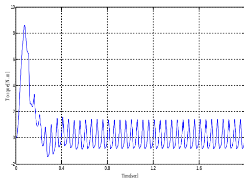
Fig.4 Electromagnetic Torque response without HF signal injection
