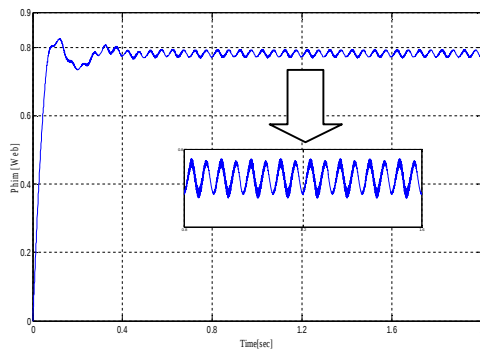
Fig.9 Magnetizing flux with HF signal injection
