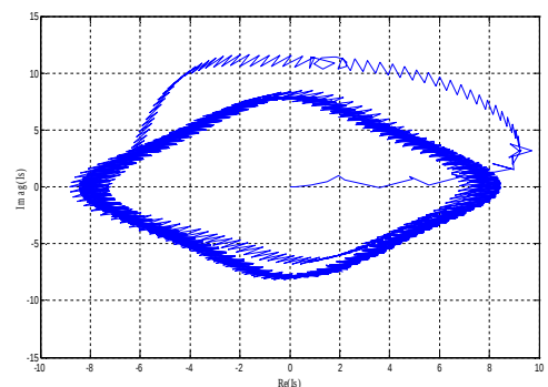
Fig.14 Phase stator current trajectory
