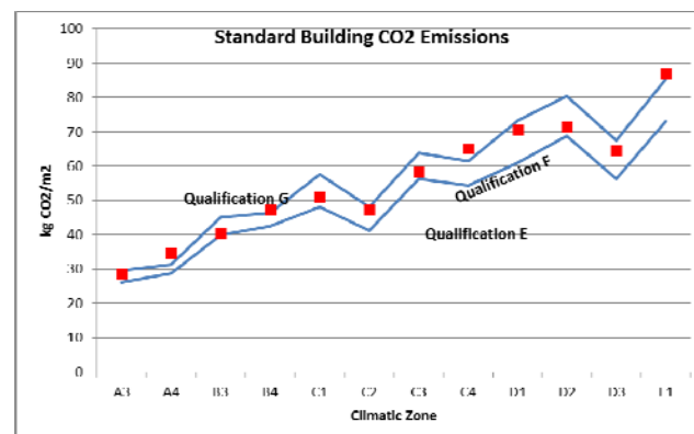
Fig. 1. – Energy performance rate and CO 2 emissions in the different Spanish climatic zones
