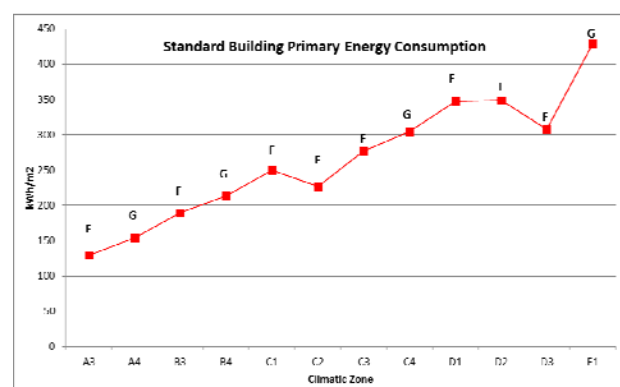
Fig. 2. - Energy performance rate and primary energy consumption in the different Spanish climatic zones
