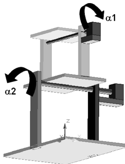
Fig. 3. Electro-Mechanical System: Axis 1 and 2
