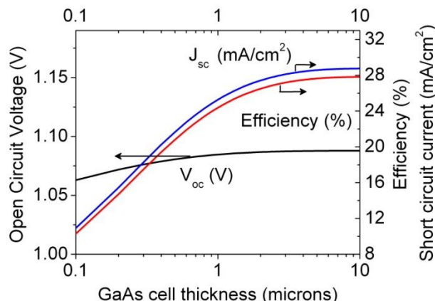
Figure 4: GaAs solar cell electrical characteristics as a function of cell thickness at T = 300 \text{ K} , 1000 \text{ W/m}^2 AM1.5d
